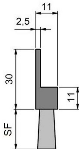
Ref. FLX6050
