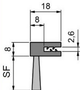
Ref. FLX1311
