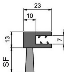
Ref. FLX1351 *
