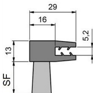
Ref. FLX1341
