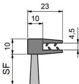
Ref. FLX1331
